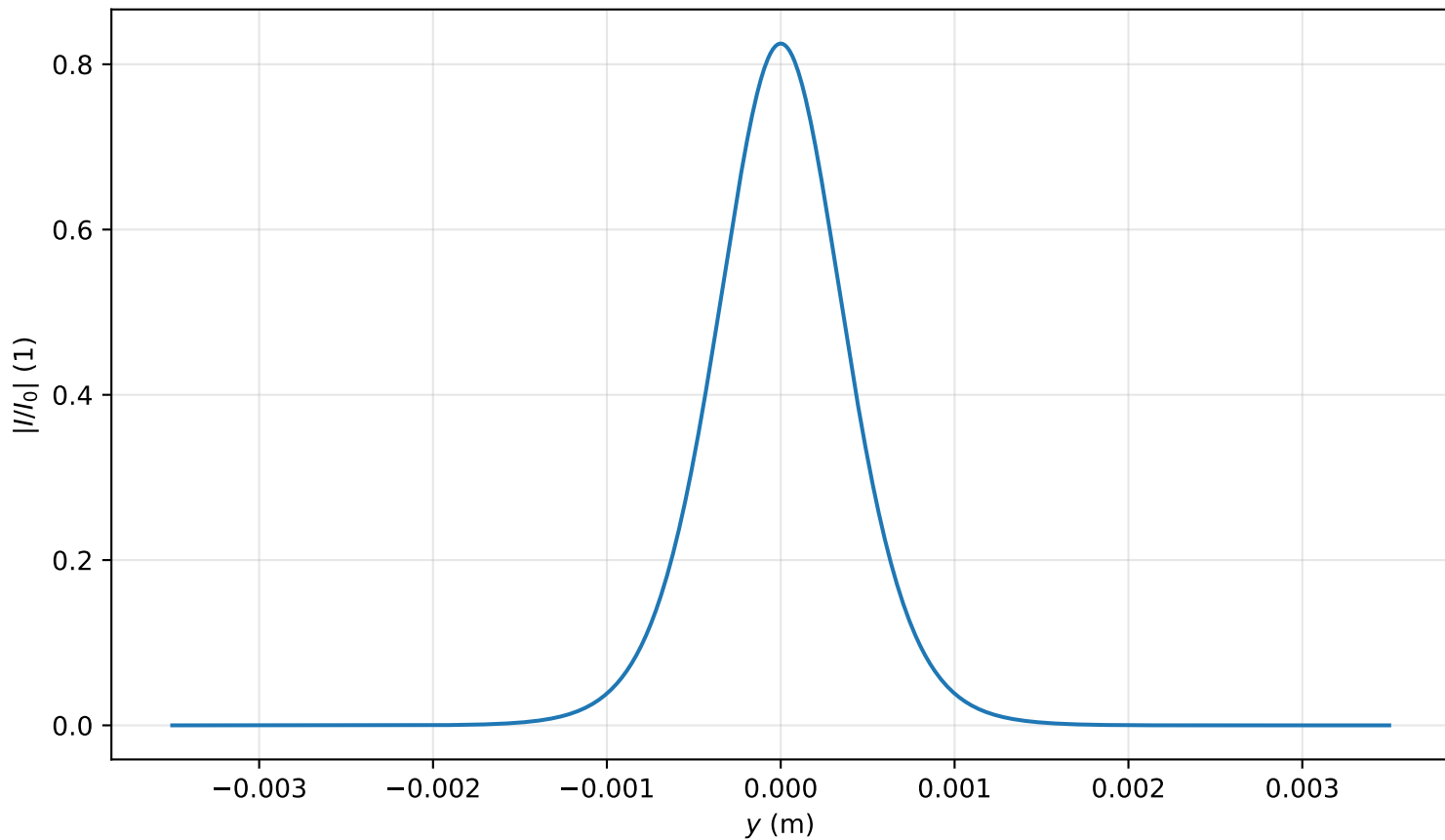
Intensity profile I(x=0, y, z=1.990)/I_0 , \text{Pin}=0.5\text{Pcr} , artificial time
